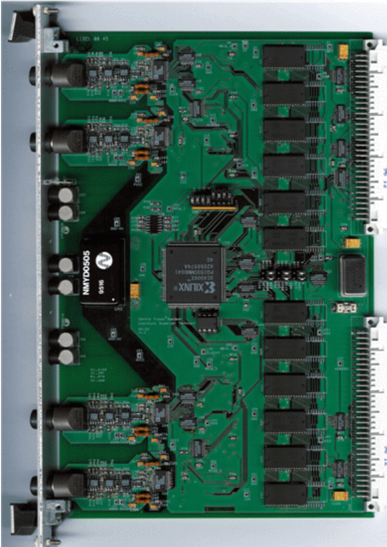
VME-AQ4-50MSPS
