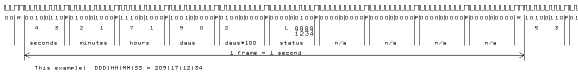
Figure 1. Pulse structure of an IRIG-B signal. (The 1KHz carrier is not displayed.)
